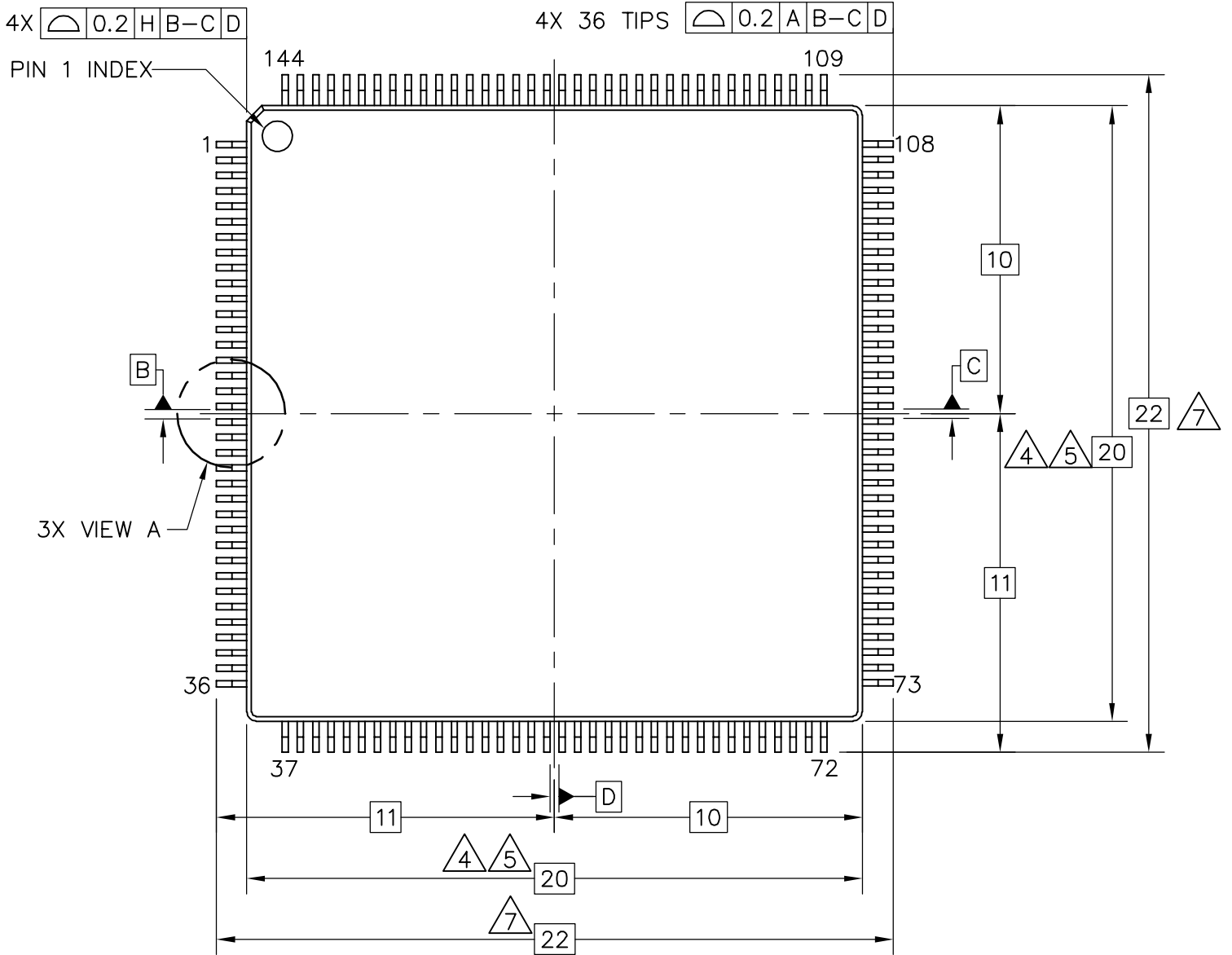
TOP VIEW
